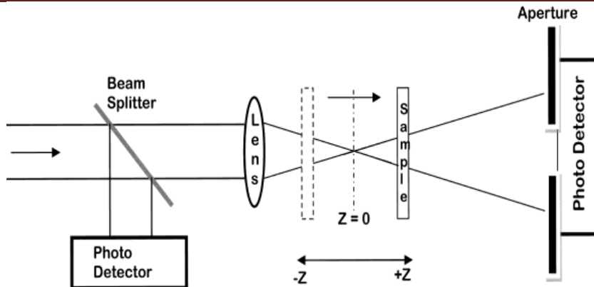
Figure 1: Schematic diagram of Z-scan experimental arrangement
