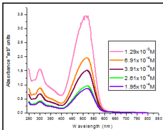
Figure 2: UV- Visible Absorption Spectra of Eriochrome Cyanine R in Solution
