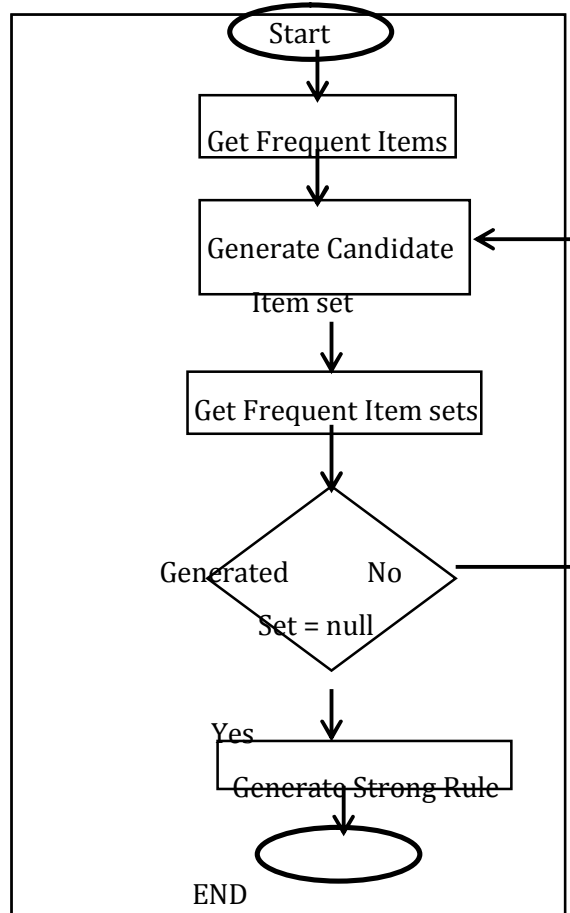
Fig 2: Apriori Flow chart
